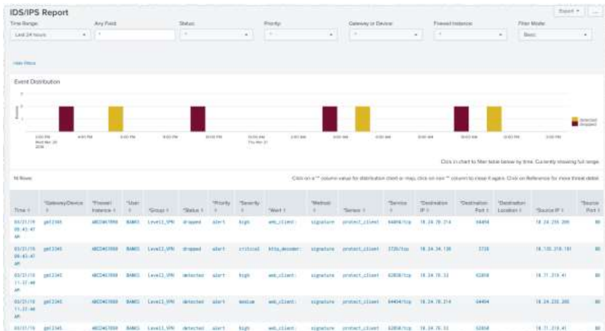
Figure 14: IDS/IPS Report
