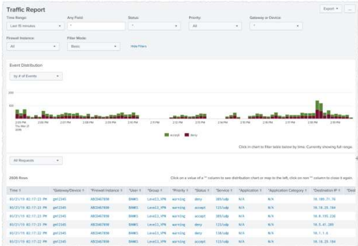
Figure 5: Traffic Report
