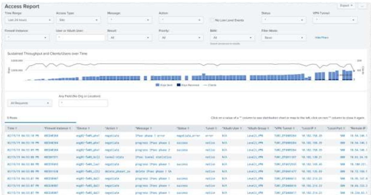
Figure 12: Access Report
